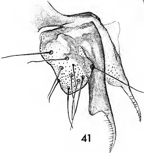
FIGS 39-42. — Lobocaecilius mouaputa , ♀ allotype : 39, fore wing; 40, subgenital plate; 41, gonapophyses; 42, epiproct. (Figs 40-42 to common scale.)
